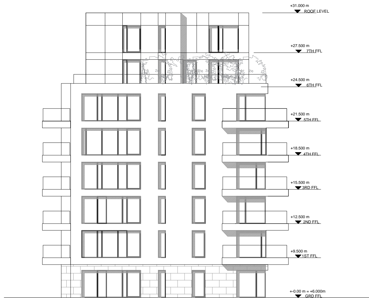
1 PROPOSED BLOCK 3 - SIDE ELEVATION 1:200
