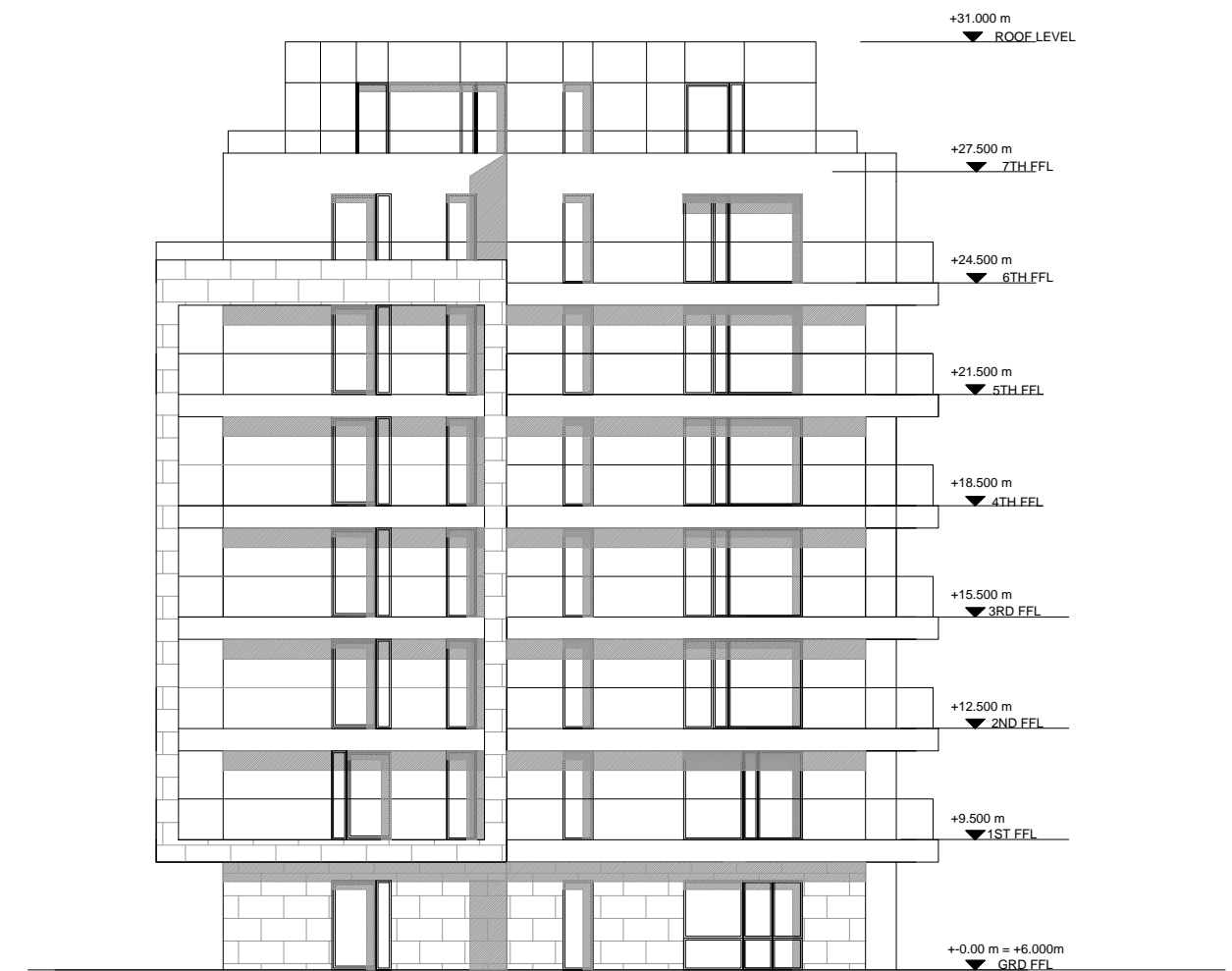
2 PROPOSED BLOCK 3 - SIDE ELEVATION 1:200
